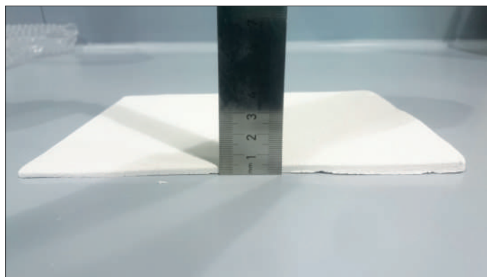
Fig. 4 Sintered alumina foam sheet with a thickness of about 4 mm, length about 290 mm, width about 210 mm
