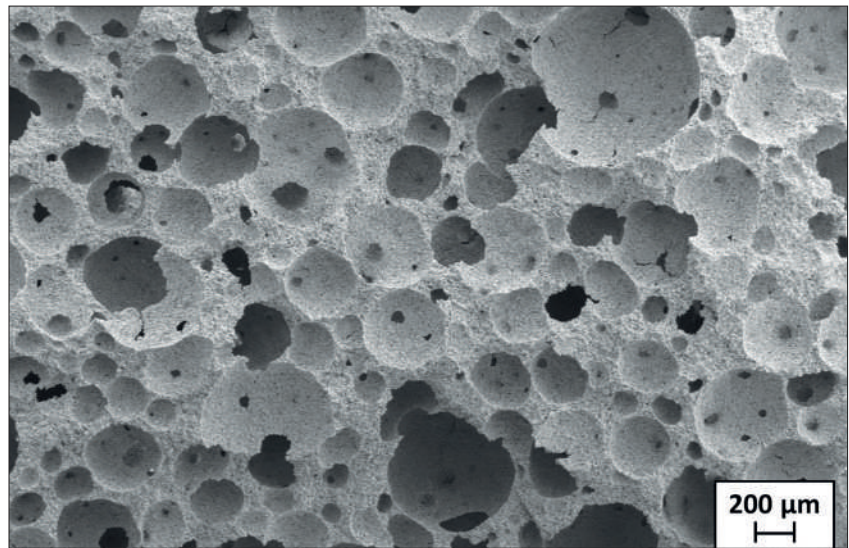
Fig. 5 SEM-picture of the microstructure of a mullite foam with a porosity of about 70 vol.-% (magnification 25 \times , working distance 15 mm, EHT 10 kV, secondary electron detector)
