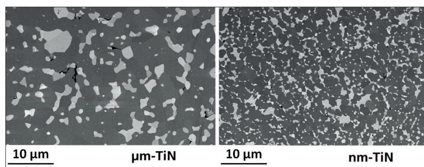
Fig. 5 SEM image (Energy Selective Backscattered (ESB)-signal) of an \text{Al}_2\text{O}_3 -TiN composite with micro-sized TiN (l.) and nano-sized TiN (r.) particles after sintering; concentration of TiN (bright phase) was 19 vol.-%
