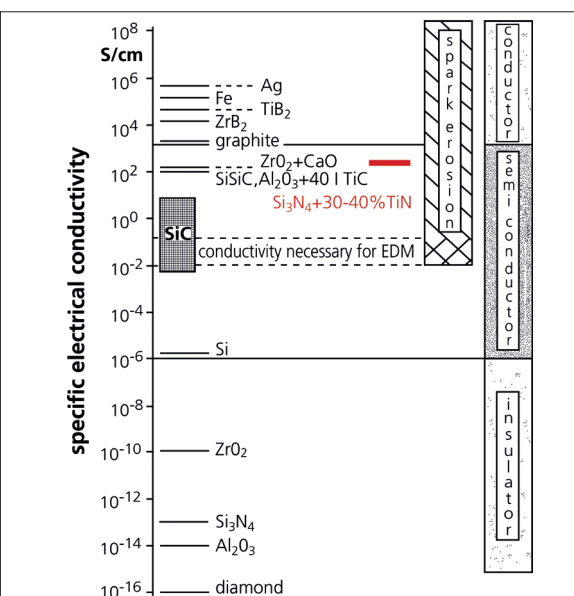
Fig. 1 Specific electrical conductivity of materials, according to [1]
