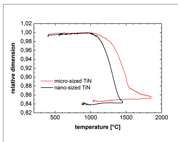
Fig. 6 Sintering curves of \text{Al}_2\text{O}_3 -composites with nano-scaled TiN in comparison to micro-scaled TiN as second phase
