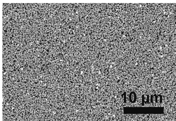
Fig. 9 Polished section of an AlN ceramic after optimised sintering
