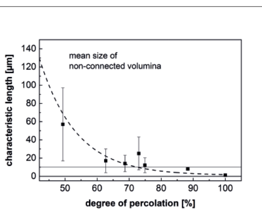
Fig. 3 Influence of the degree of percolation on the mean size of non-contacted volume
